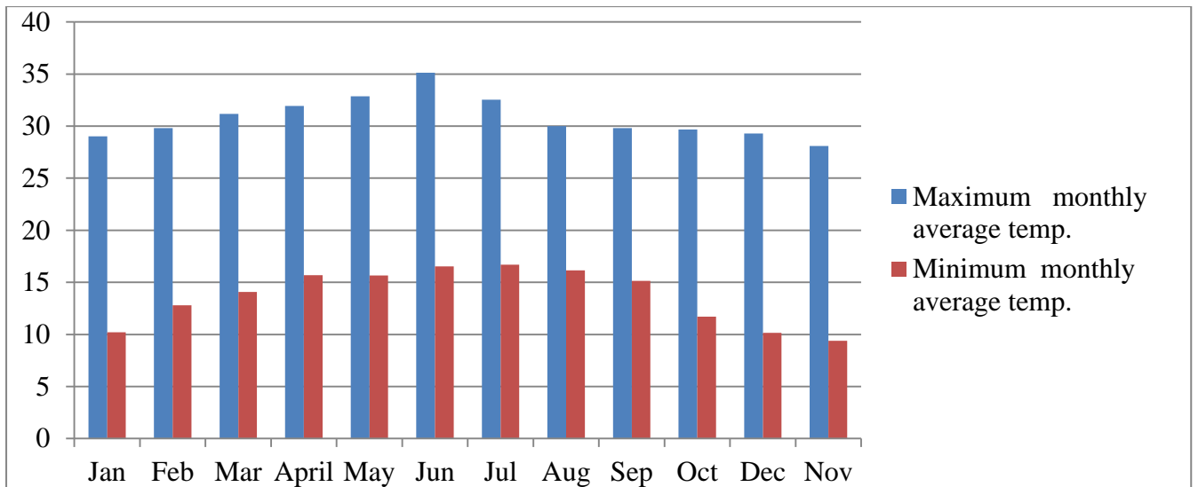
Figure 2. Monthly average temperature of Dewacheffa District ( 2011 to 2020 )
