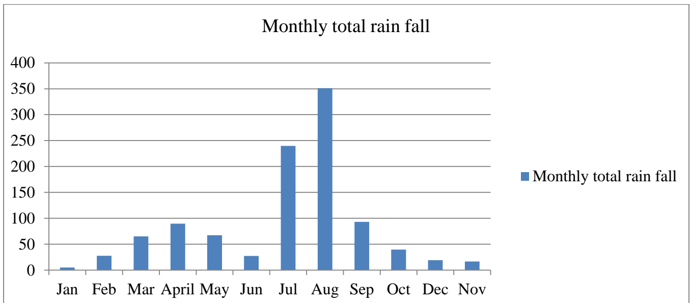
Figure 3. Mean monthly distribution of rain fall in dewacheffa ( 2011 to 2020)
